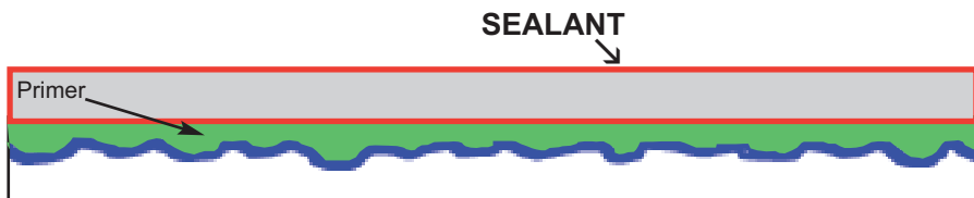
Fig 1d Primed surface – good contact
