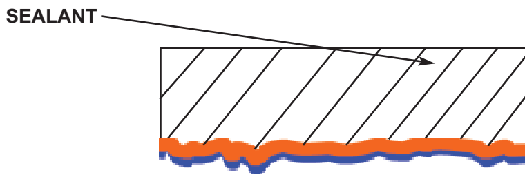
Fig.1b Smooth surface (magnified) - good contact
